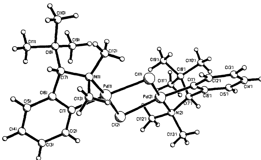
Figure 1. X-Ray structure of dimer ( S_C )- 1e . C_{26}H_{40}Cl_2N_2Pd_2 , M 664.36, orthorhombic space group P2_12_12_1 , a 10.640(3), b 12.126(4), c 22.496(7) Å, V 2902(2) Å 3 , Z 4, D_x 1.520 g cm -3 , Mo- K\alpha radiation, 1.071073 Å, \mu (Mo- K\alpha ) 14.39 cm -1 ; 293 K; the final R and R_w values are 0.0349 and 0.0694, respectively, for 2836 independent reflections corrected for absorption by \Psi -scan curve.
