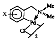
Figure 1. X-Ray structure of dimer ( S_C )- 1e . C_{26}H_{40}Cl_2N_2Pd_2 , M 664.36, orthorhombic space group P2_12_12_1 , a 10.640(3), b 12.126(4), c 22.496(7) Å, V 2902(2) Å 3 , Z 4, D_x 1.520 g cm -3 , Mo- K\alpha radiation, 1.071073 Å, \mu (Mo- K\alpha ) 14.39 cm -1 ; 293 K; the final R and R_w values are 0.0349 and 0.0694, respectively, for 2836 independent reflections corrected for absorption by \Psi -scan curve.
